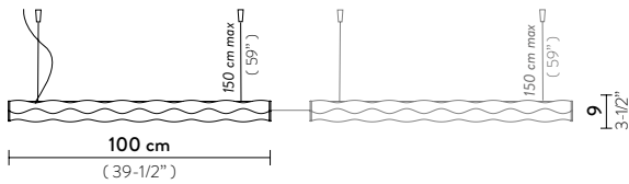
1 X HUGO MAIN electrified module CE IP 20
